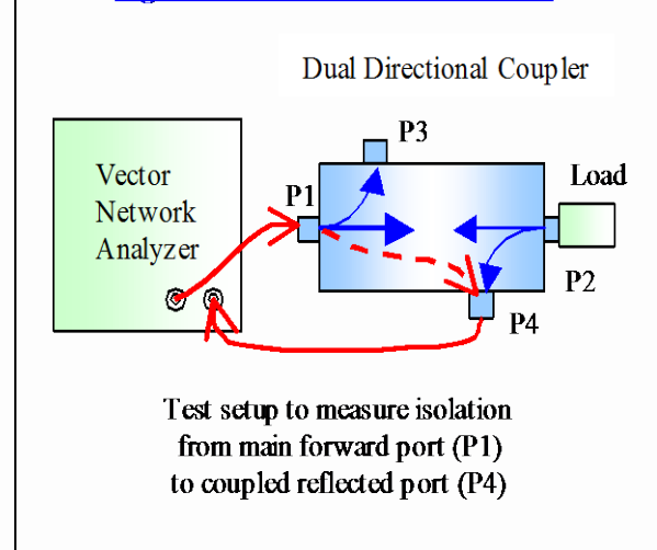
Figure 2: Isolation Measurement
