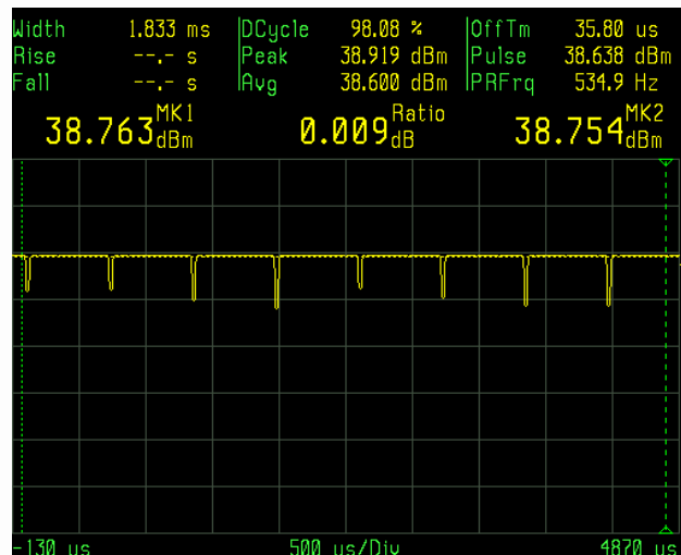
Figure 1: GSM Waveform with All Time Slots Open
