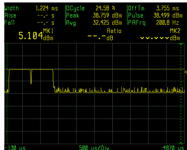
Figure 2: GSM Waveform with 2 Time Slots Open
