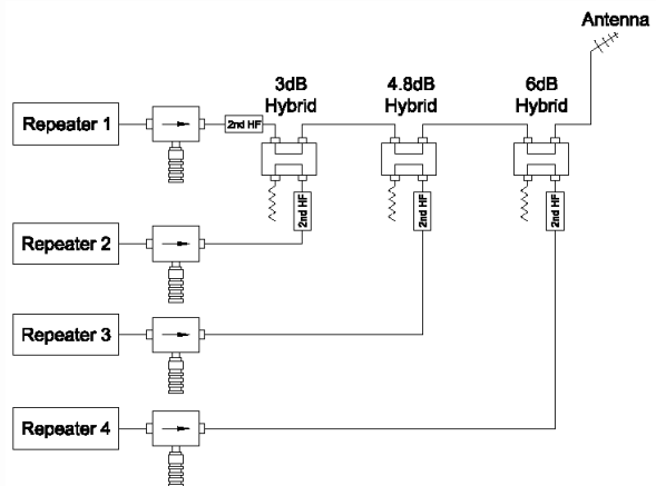
Figure 3. 4-Channel Progressive Hybrid Combiner Approximately 7dB Loss Per Channel
