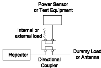
Figure 2b. Hybrid Sampler configured to measure Reflected power
