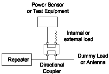
Figure 2a. Hybrid Sampler configured to measure Incident power
