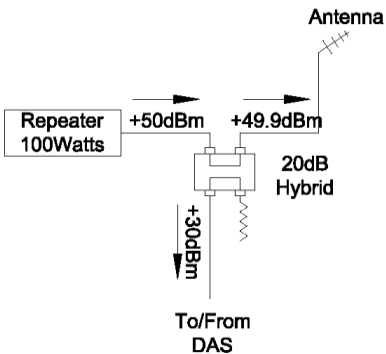
Figure 2c. Hybrid Coupled Repeater
